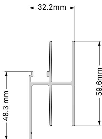
CB-LIFE profilo passata CB-LIFE pass frame
