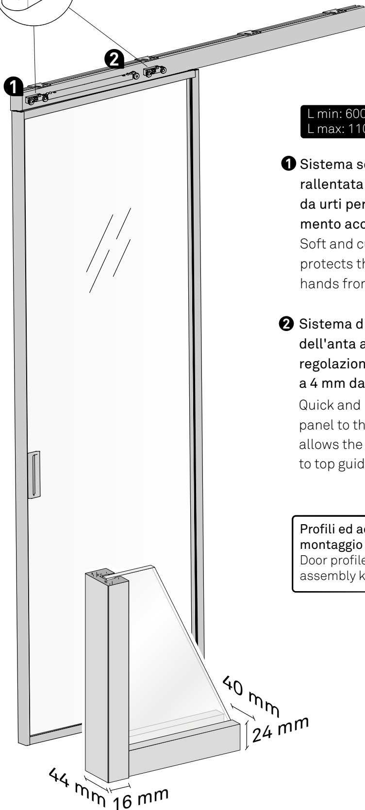
KIT AGGANCIO ANTA DOOR COUPLING KIT
